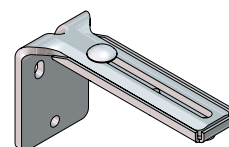
Justerbar vinkel, 55-110 mm 35/50/70 mm
